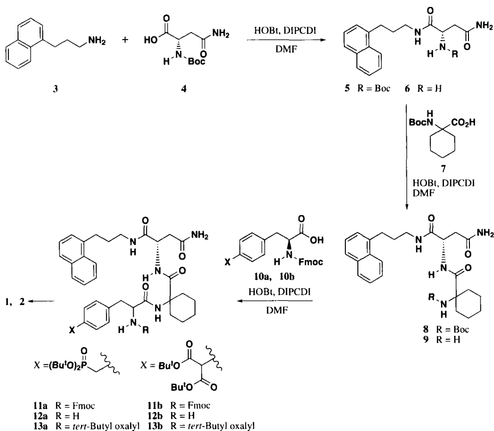
Scheme 1
